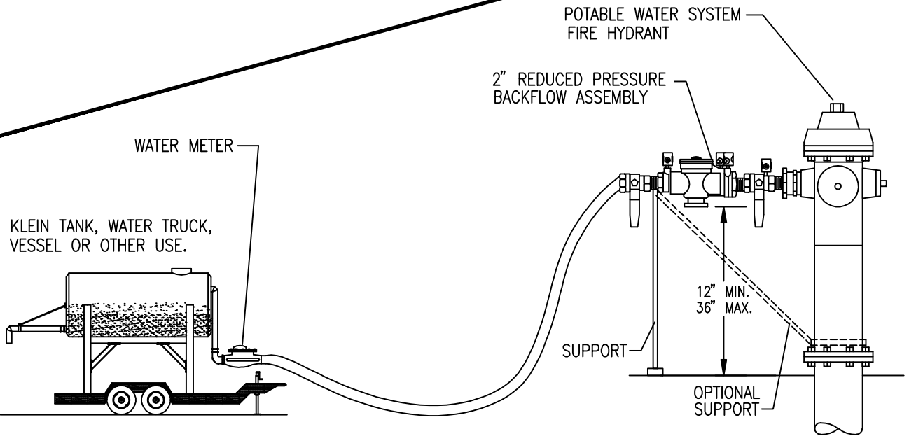
HYDRANT MOUNTED RP BACKFLOW ASSEMBLY AND REMOTE METER
