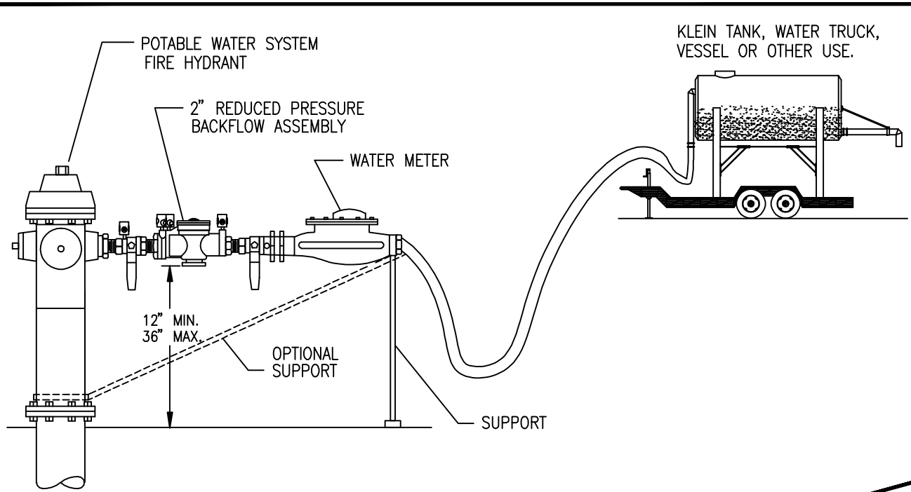
HYDRANT MOUNTED RP BACKFLOW ASSEMBLY AND WATER METER
