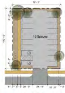
Double Loaded Parking Lot 1" = 30'
