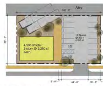
2 Story Building w/ Double Loaded Side Parking, Trash Enclosure & Alley Access 1" = 30'
