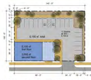
2 Story Building w/ Covered Entry Plaza & Single Loaded Parking Around 1" = 30'
