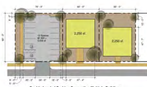
Double Loaded Parking Supporting Multiple Buildings 1" = 30'
