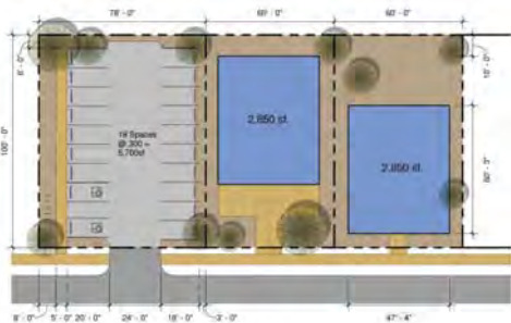
Double Loaded Parking Supporting Multiple Buildings 1" = 30'
