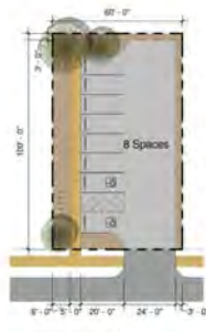
Single Loaded Parking Lot 1" = 30'
