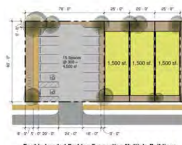
Double Loaded Parking Supporting Multiple Buildings 1" = 30'
