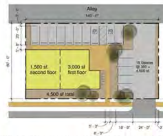
2 Story Building w/ Single Loaded Side & Alley Access Parking 1" = 30'
