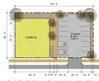
Single Story Building w/ Double Loaded parking @ Side 1" = 30'
