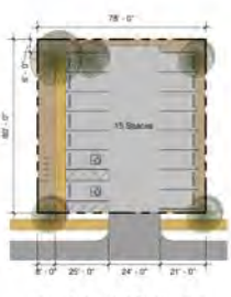
Double Loaded Parking Lot 1" = 30'
