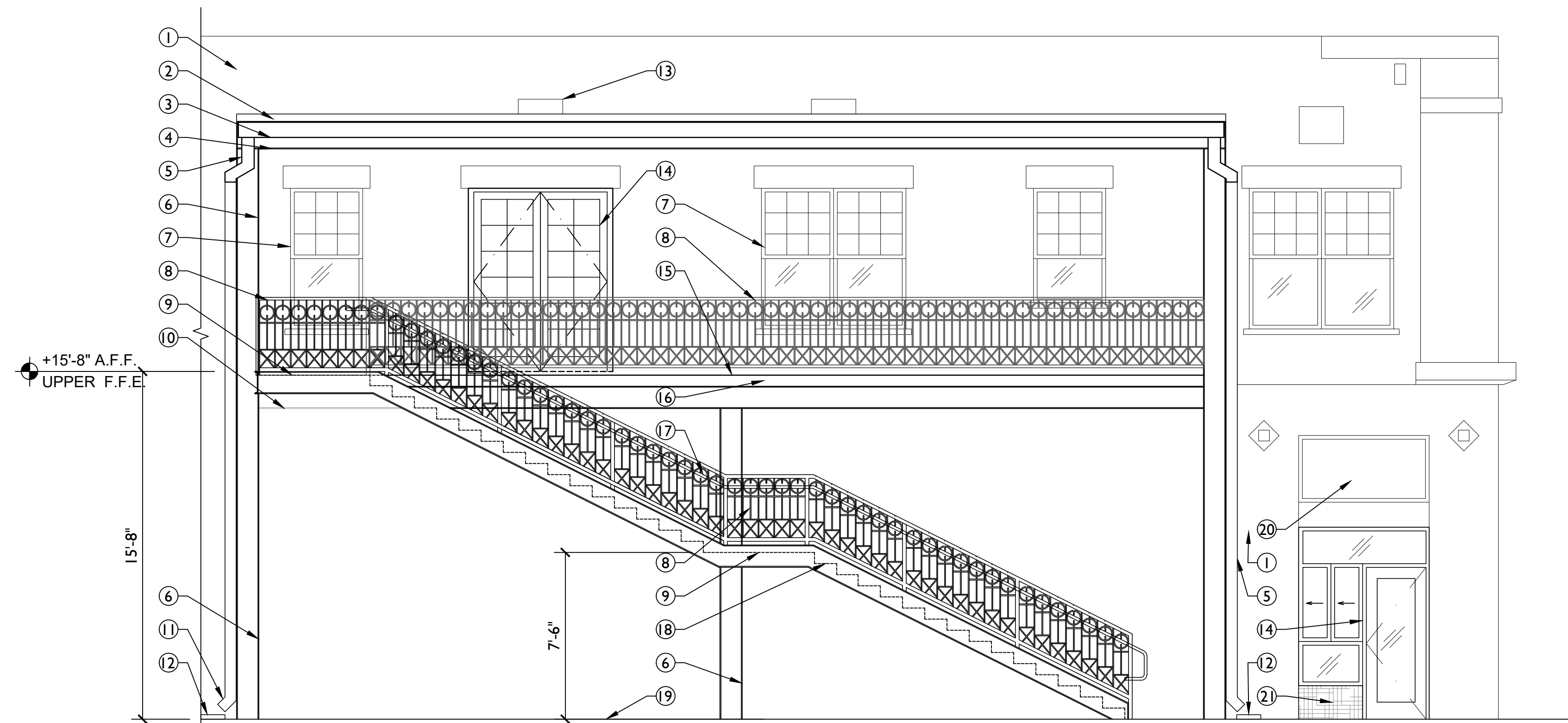
2 EAST ELEVATION SCALE 1/4" = 1'-0"
