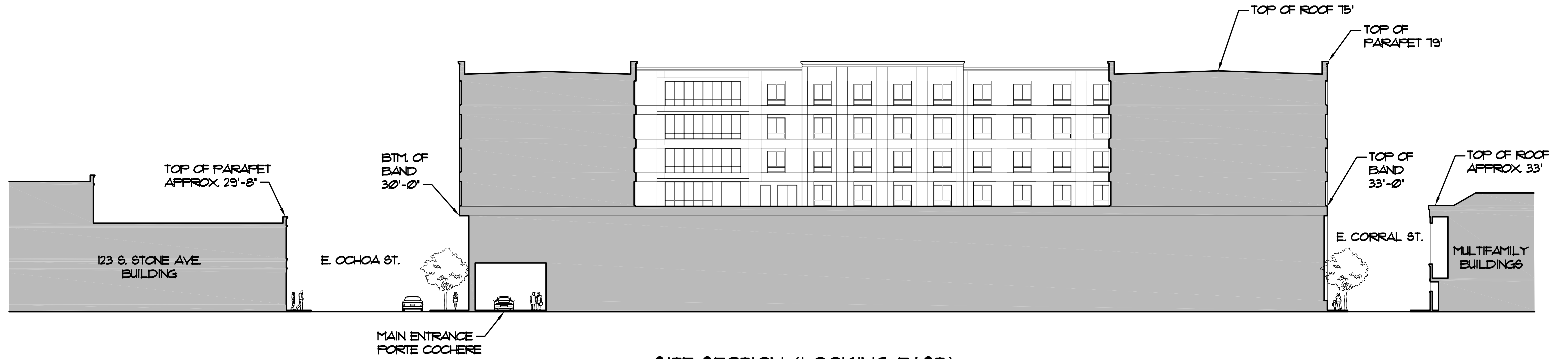
SITE SECTION (LOOKING EAST)
