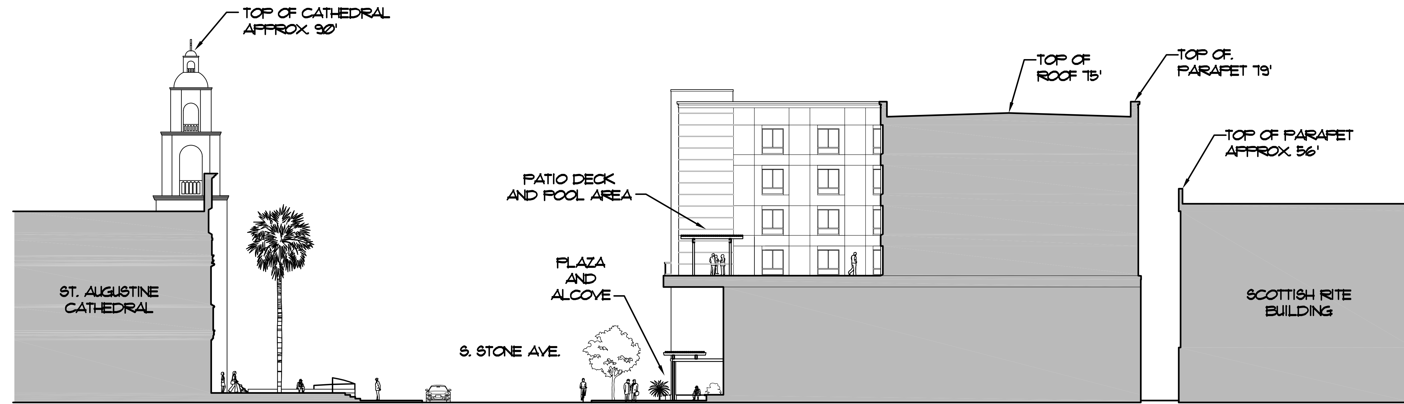
SITE SECTION (LOOKING NORTH)
