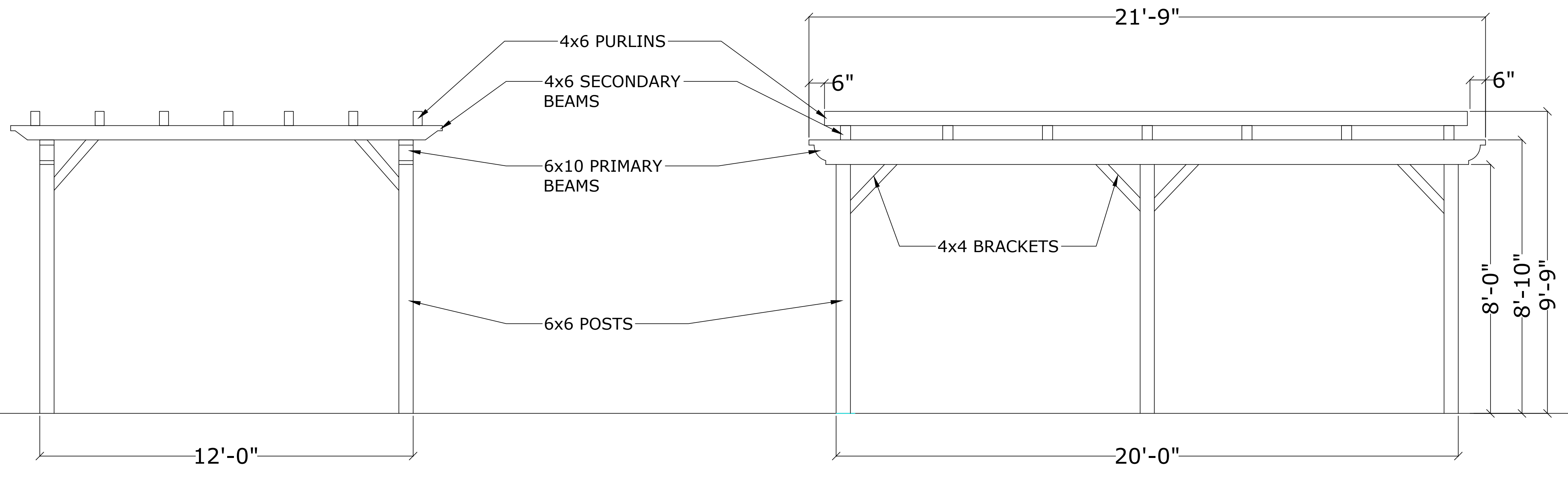
1 RAMADA ELEVATIONS SCALE: 3/4"=1'-0"
