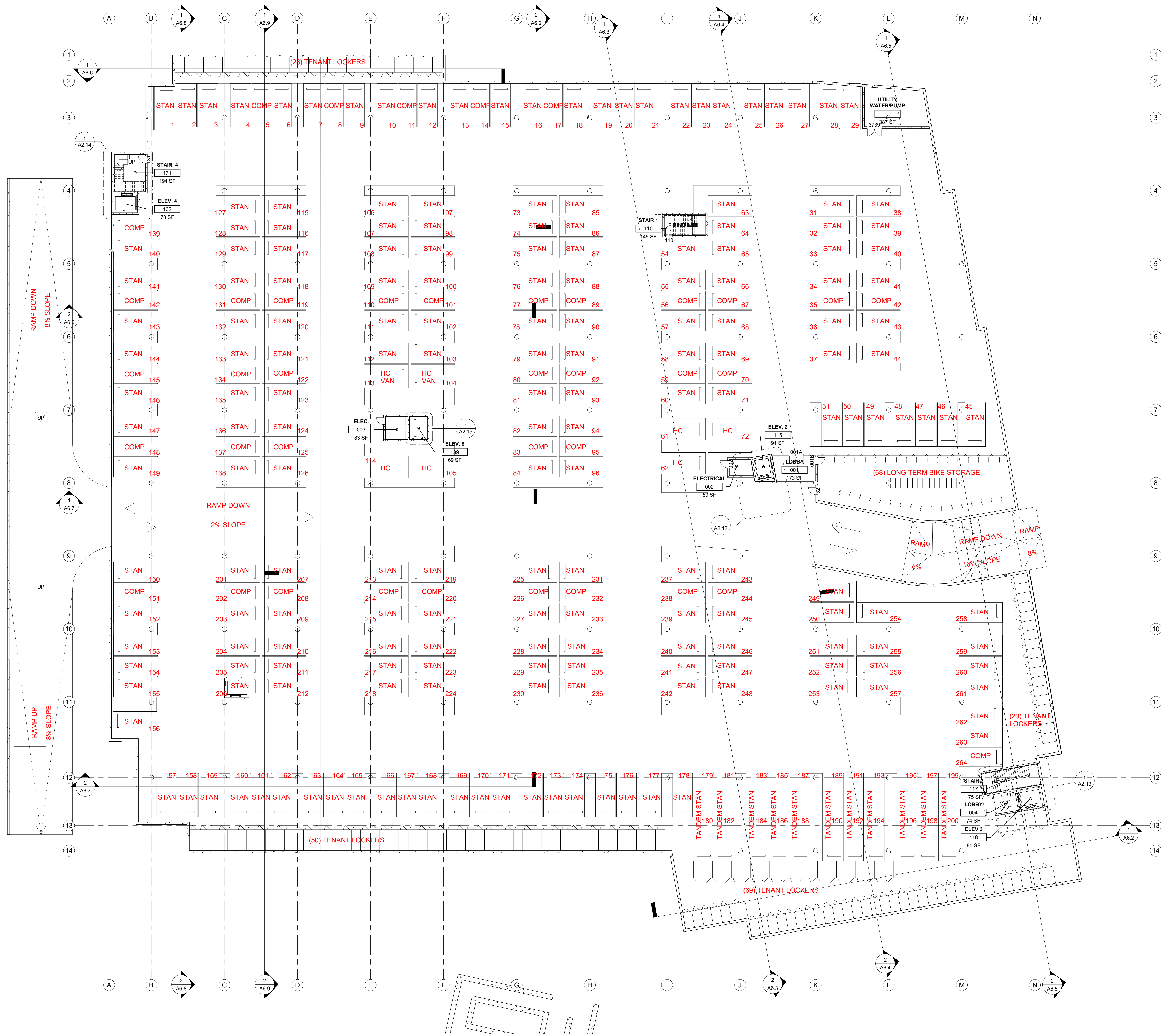
1 GARAGE FLOOR PLAN SCALE: 1/16" = 1'-0"
