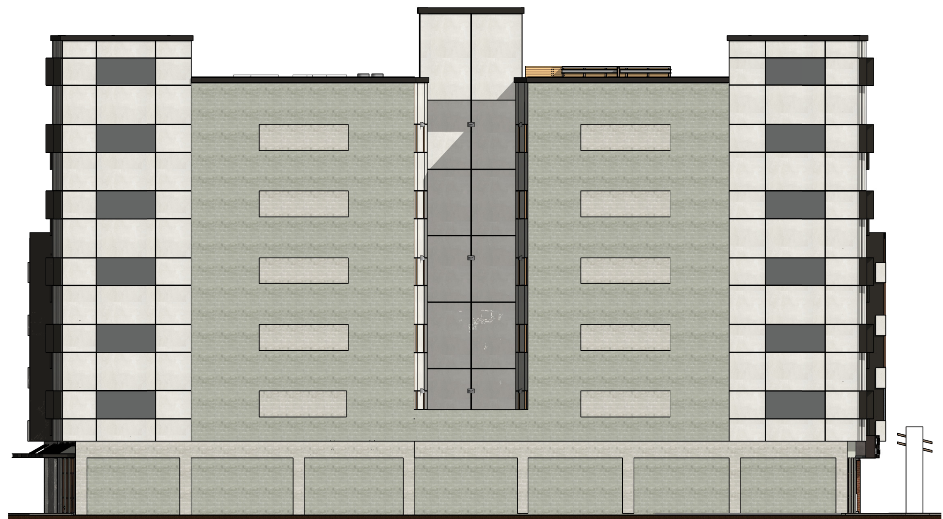
East Elevation
