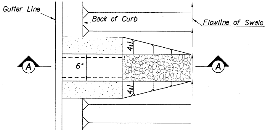
PLAN 6"x 6" Steel Tube
