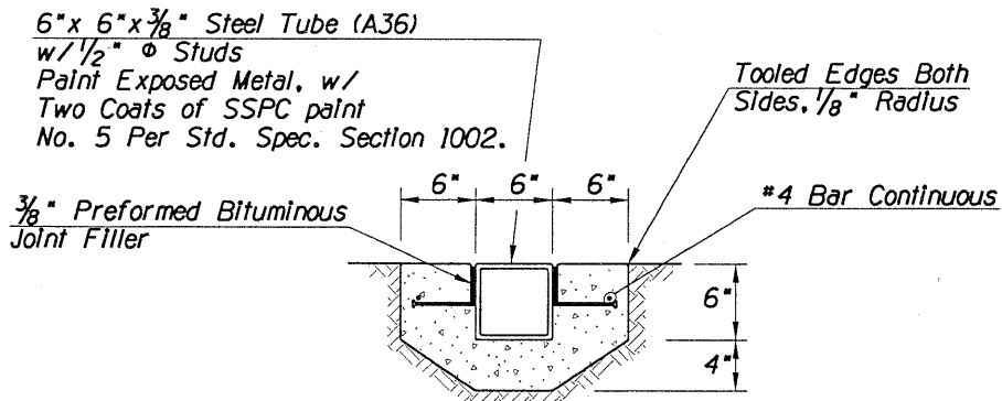
SECTION B-B 6"x 6" Steel Tube
