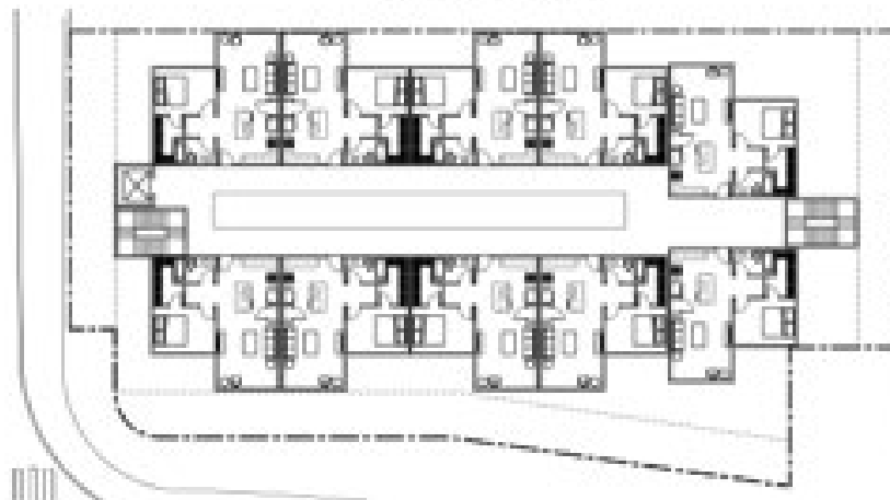
6TH FLOOR - 8 UNITS
