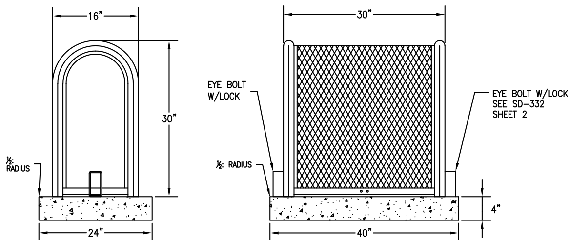
GUARD SHACK #3.3 (16"W X 30"H X 30"L) QUALITY ENCLOSURE #3.3 (16"W X 30"H X 30"L)
