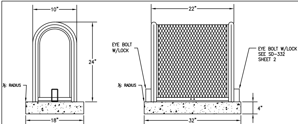
GUARD SHACK #1 (10"W X 24"H X 22"L) QUALITY ENCLOSURE #1 (10"W X 24"H X 22"L)
