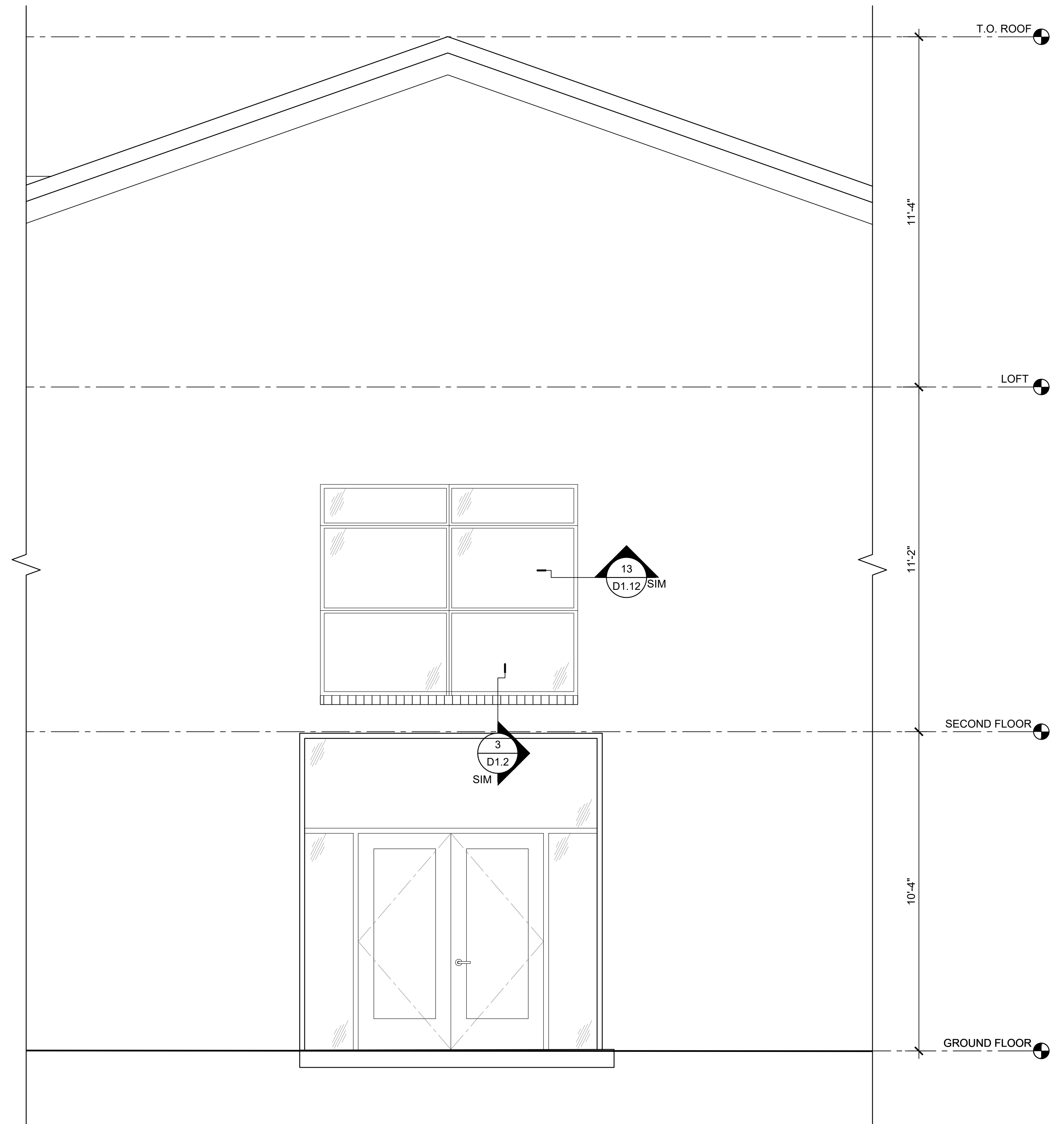
1 BUILDING 5 ELEVATION - SOUTH SCALE: 1/2"=1'-0"
