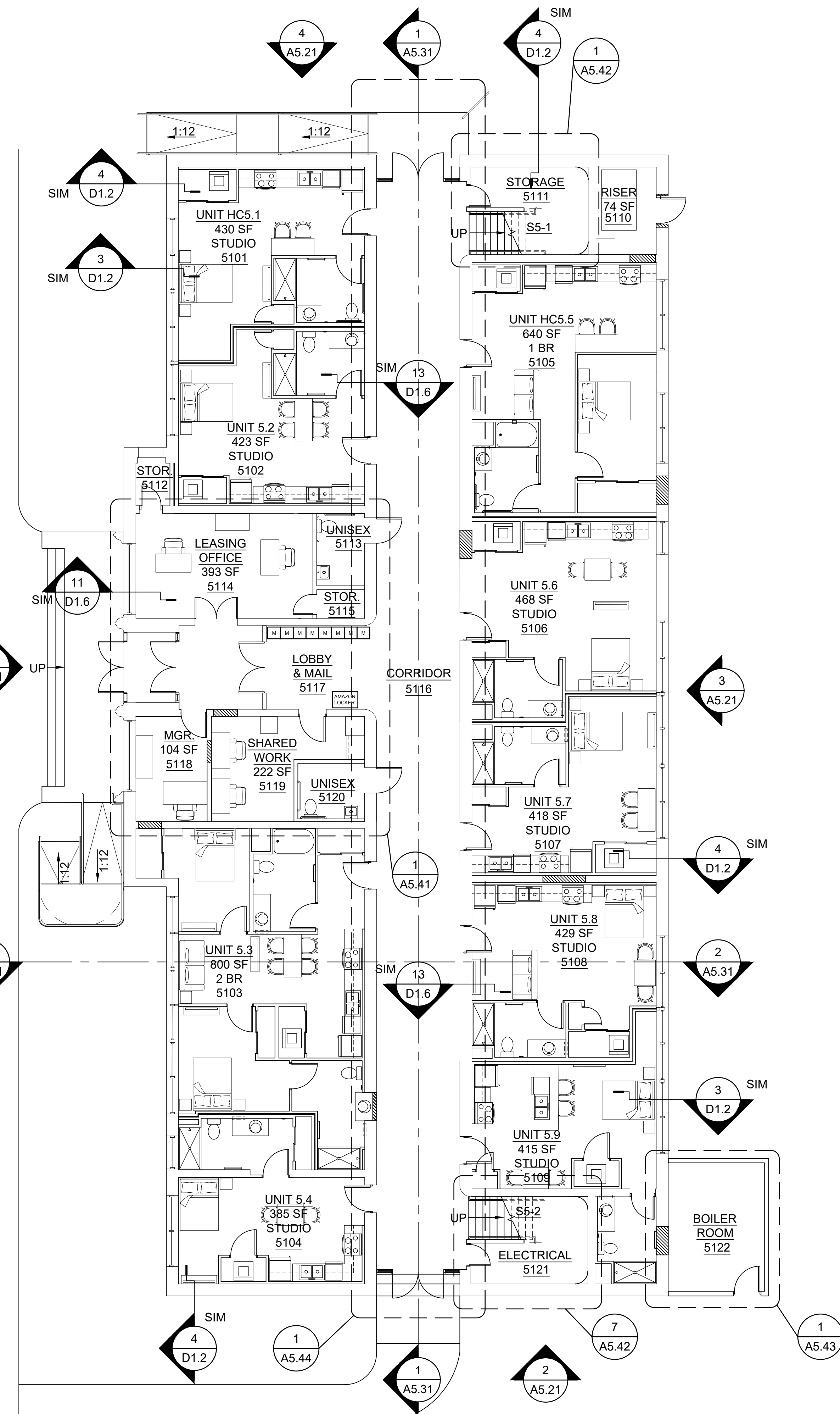
1 GROUND FLOOR PLAN SCALE: 1/8"=1'-0"
