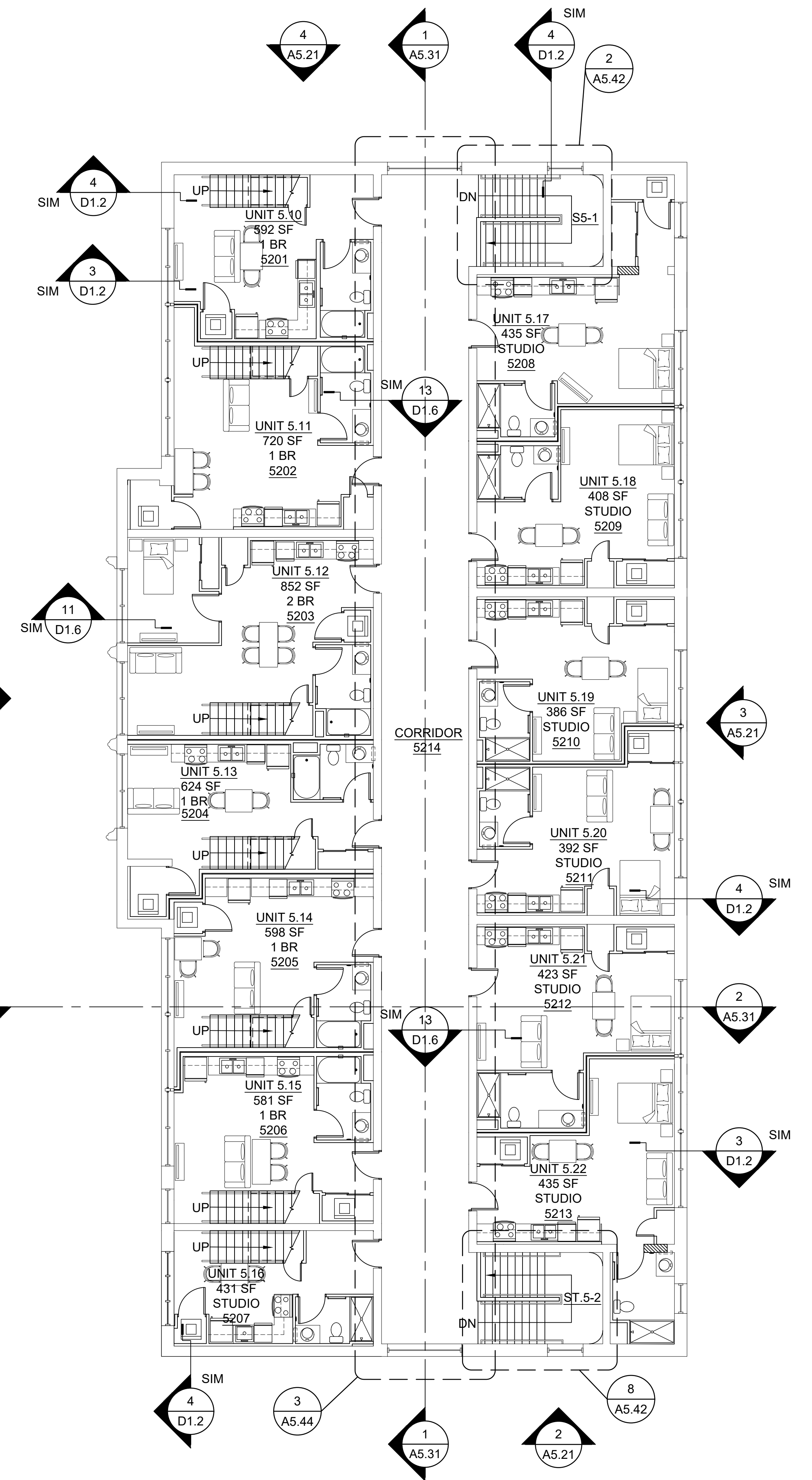
2 SECOND FLOOR PLAN SCALE: 1/8"=1'-0"
