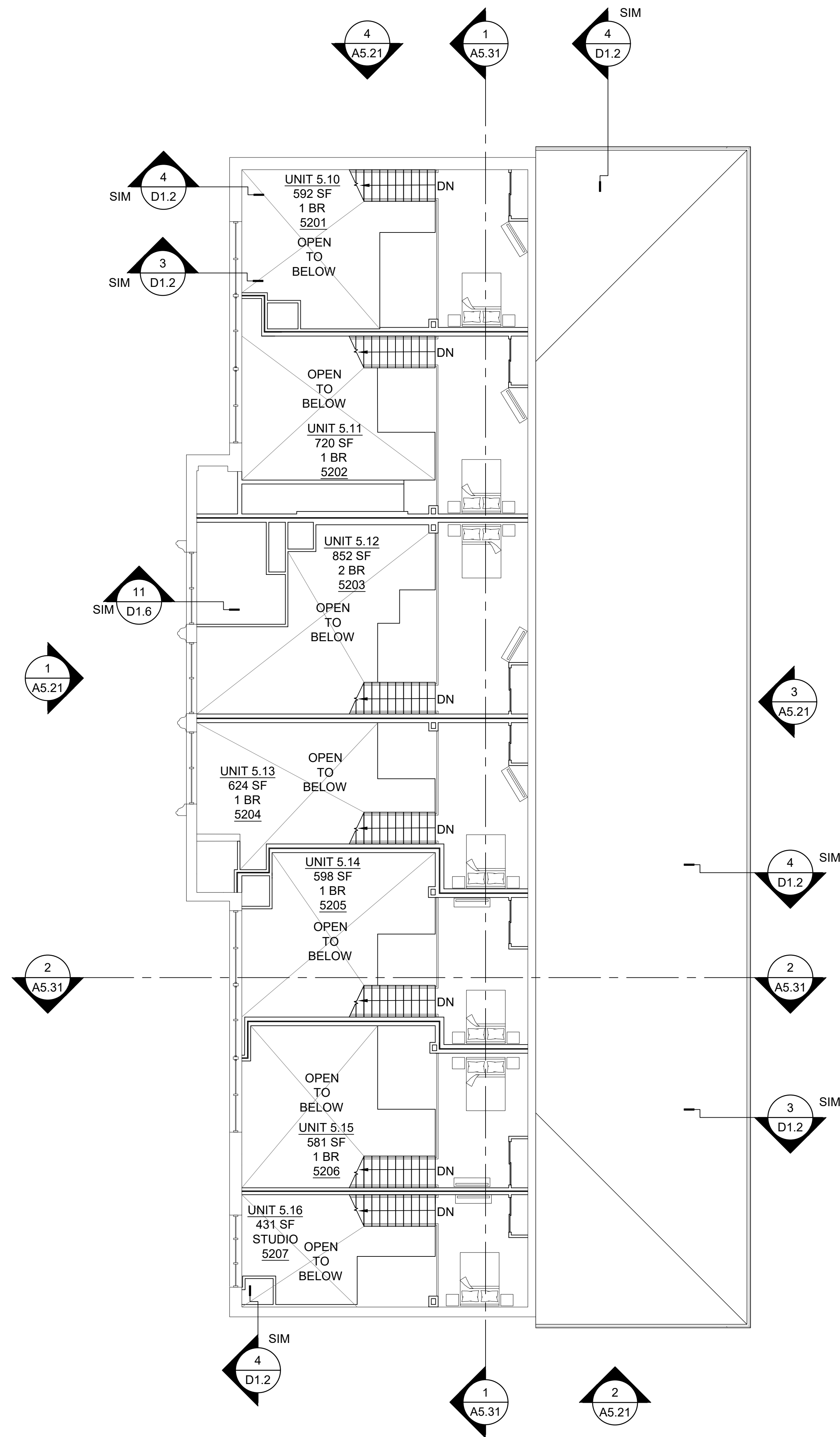
3 LOFT LEVEL FLOOR PLAN SCALE: 1/8"=1'-0"
