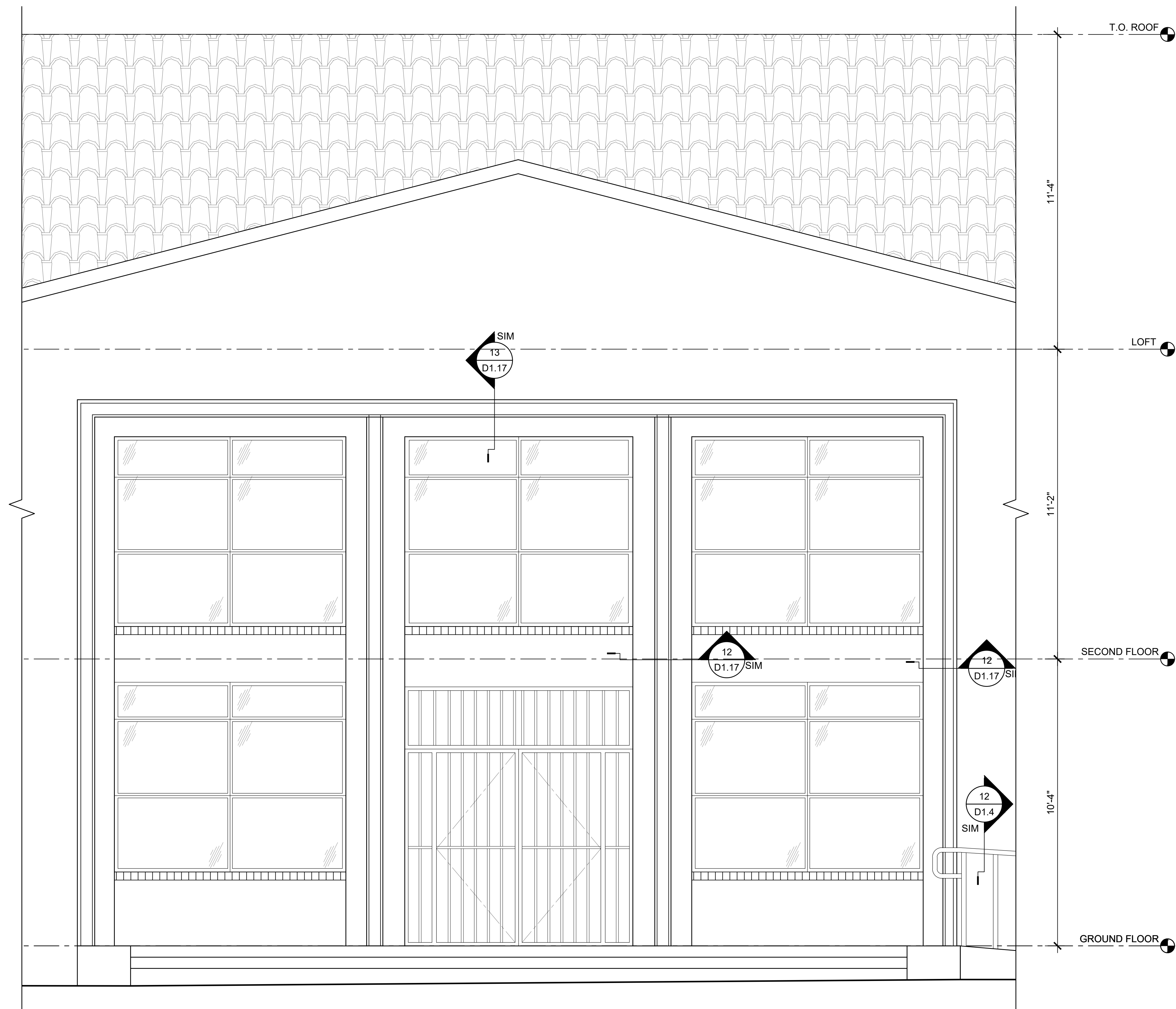
2 BUILDING 5 ELEVATION - WEST SCALE: 1/2"=1'-0"
