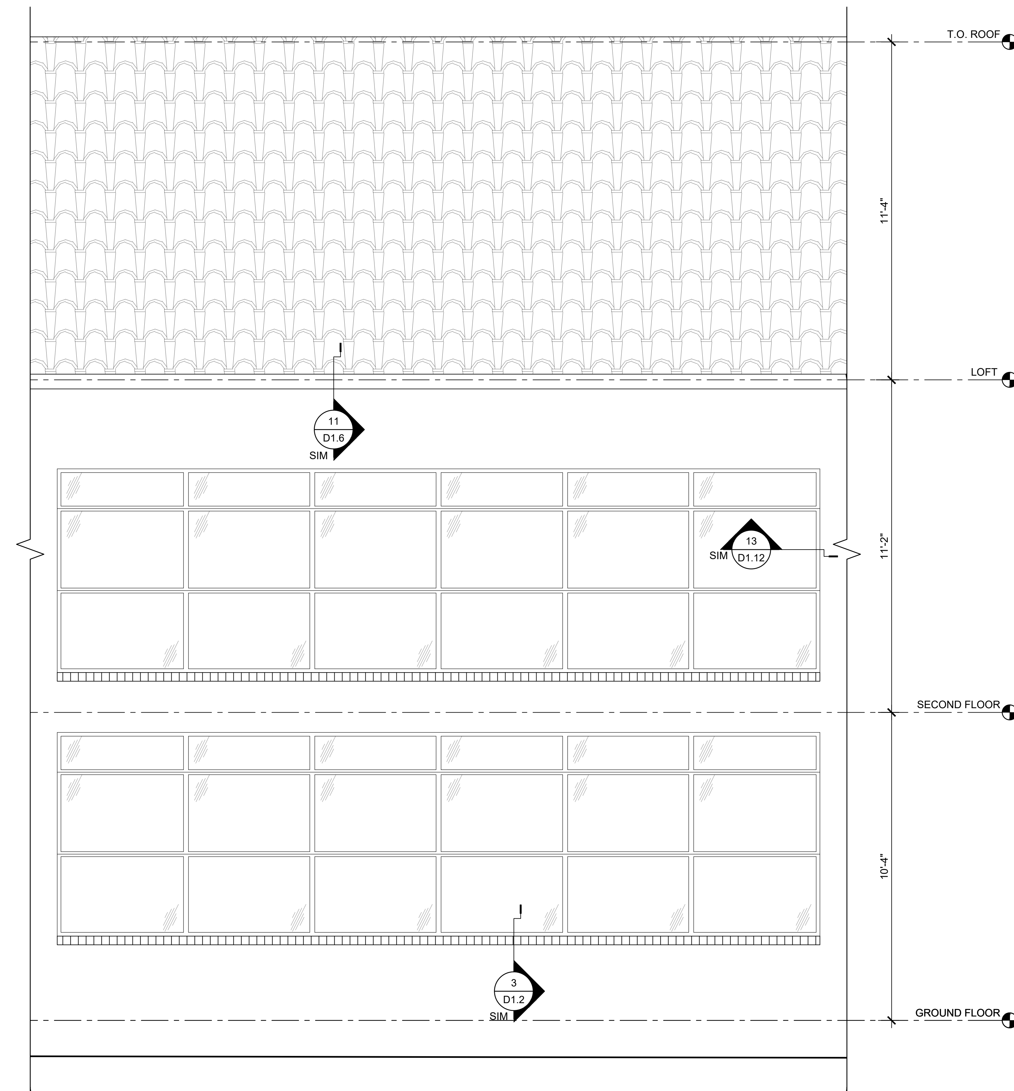
1 BUILDING 5 ELEVATION - WEST SCALE: 1/2"=1'-0"
