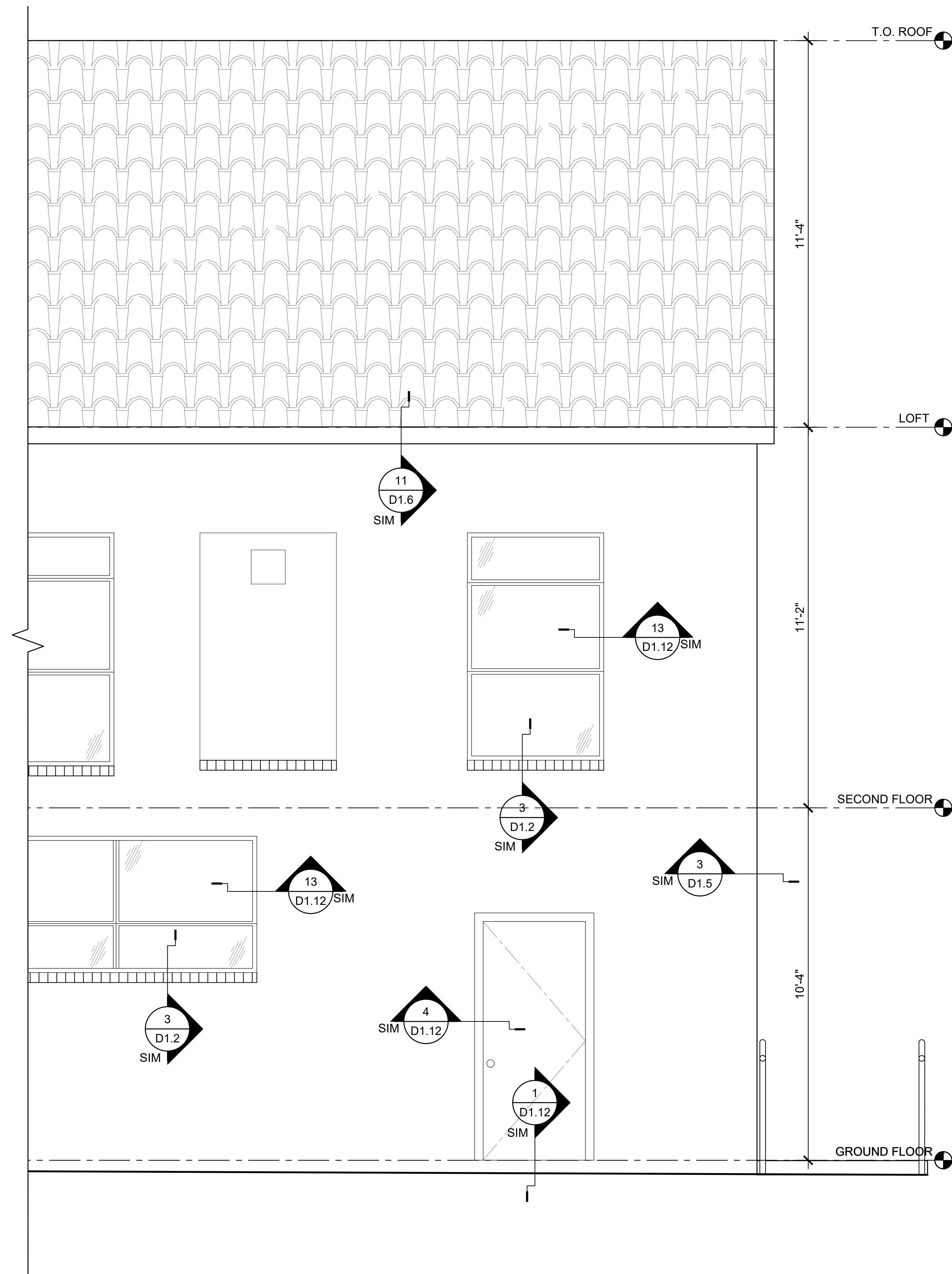
2 BUILDING 5 ELEVATION - EAST SCALE: 1/2"=1'-0"
