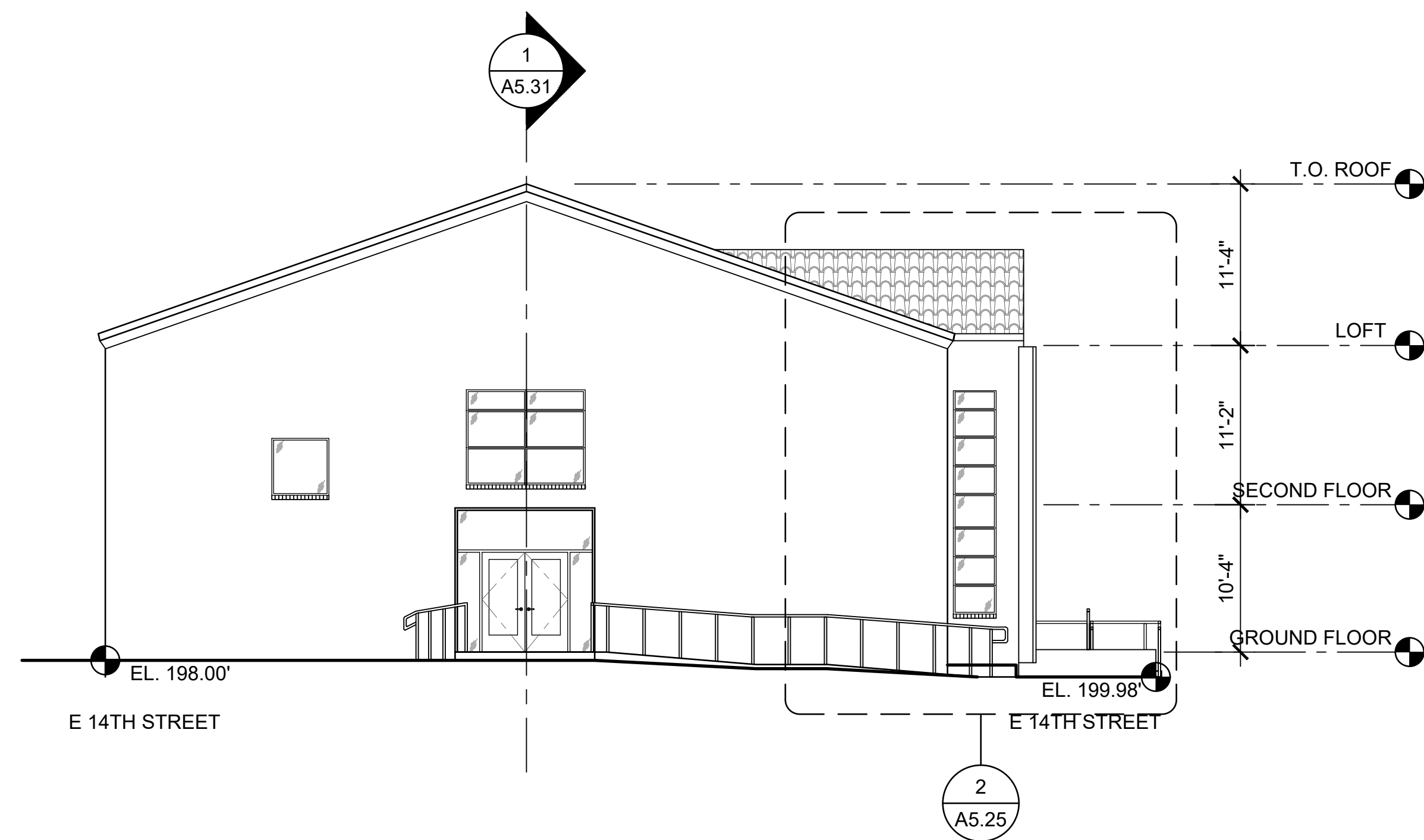
4 BUILDING 5 ELEVATION - NORTH SCALE: 1/8"=1'-0"
