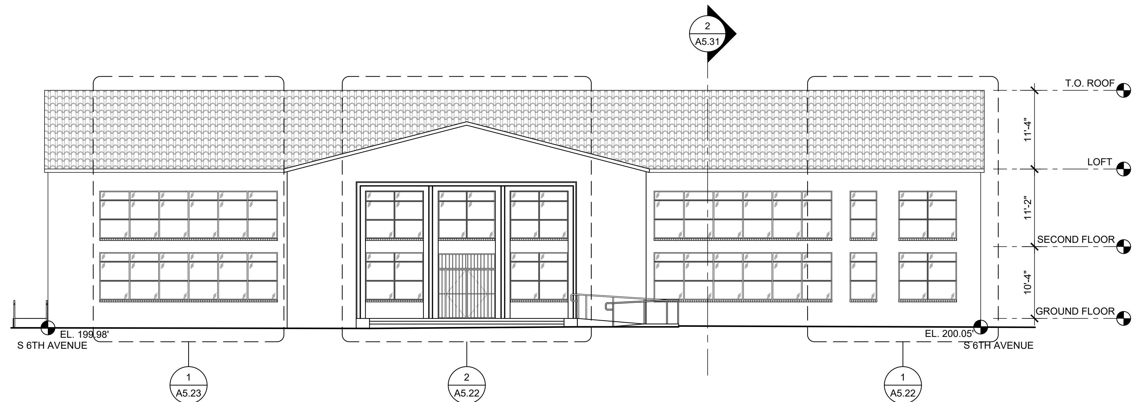
1 BUILDING 5 ELEVATION - WEST SCALE: 1/8"=1'-0"
