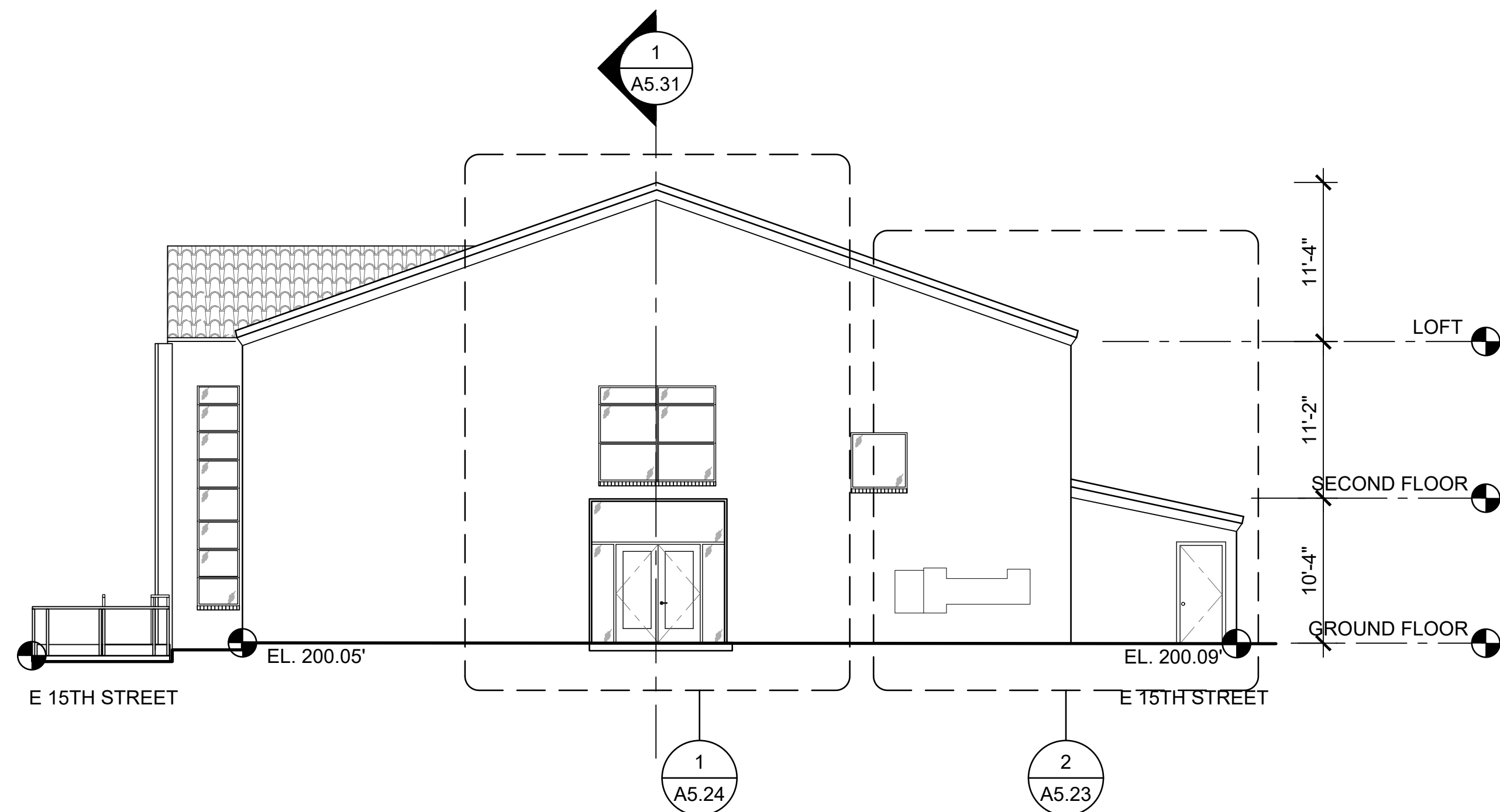
2 BUILDING 5 ELEVATION - SOUTH SCALE: 1/8"=1'-0"
