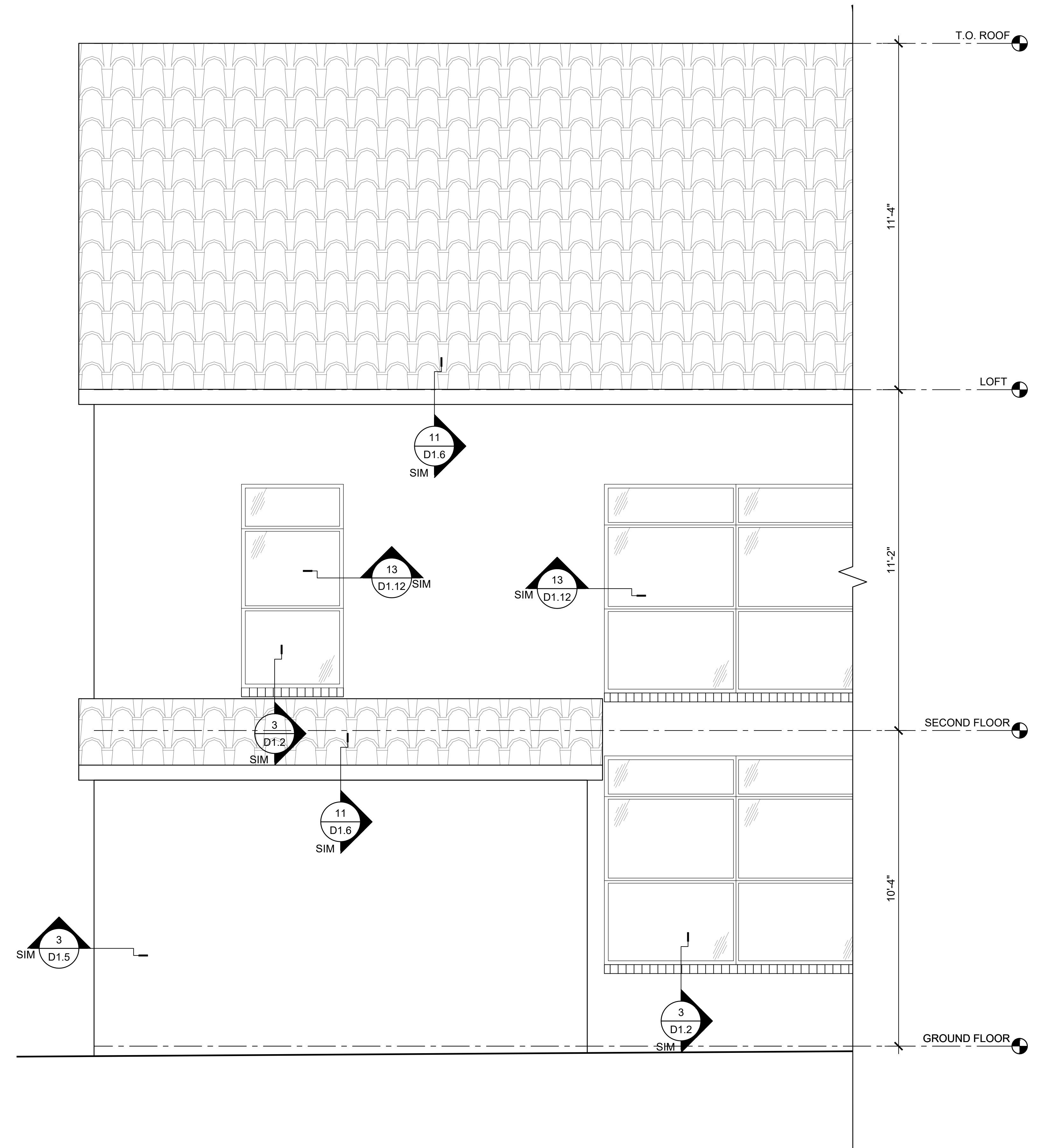
1 BUILDING 5 ELEVATION - EAST SCALE: 1/2"=1'-0"
