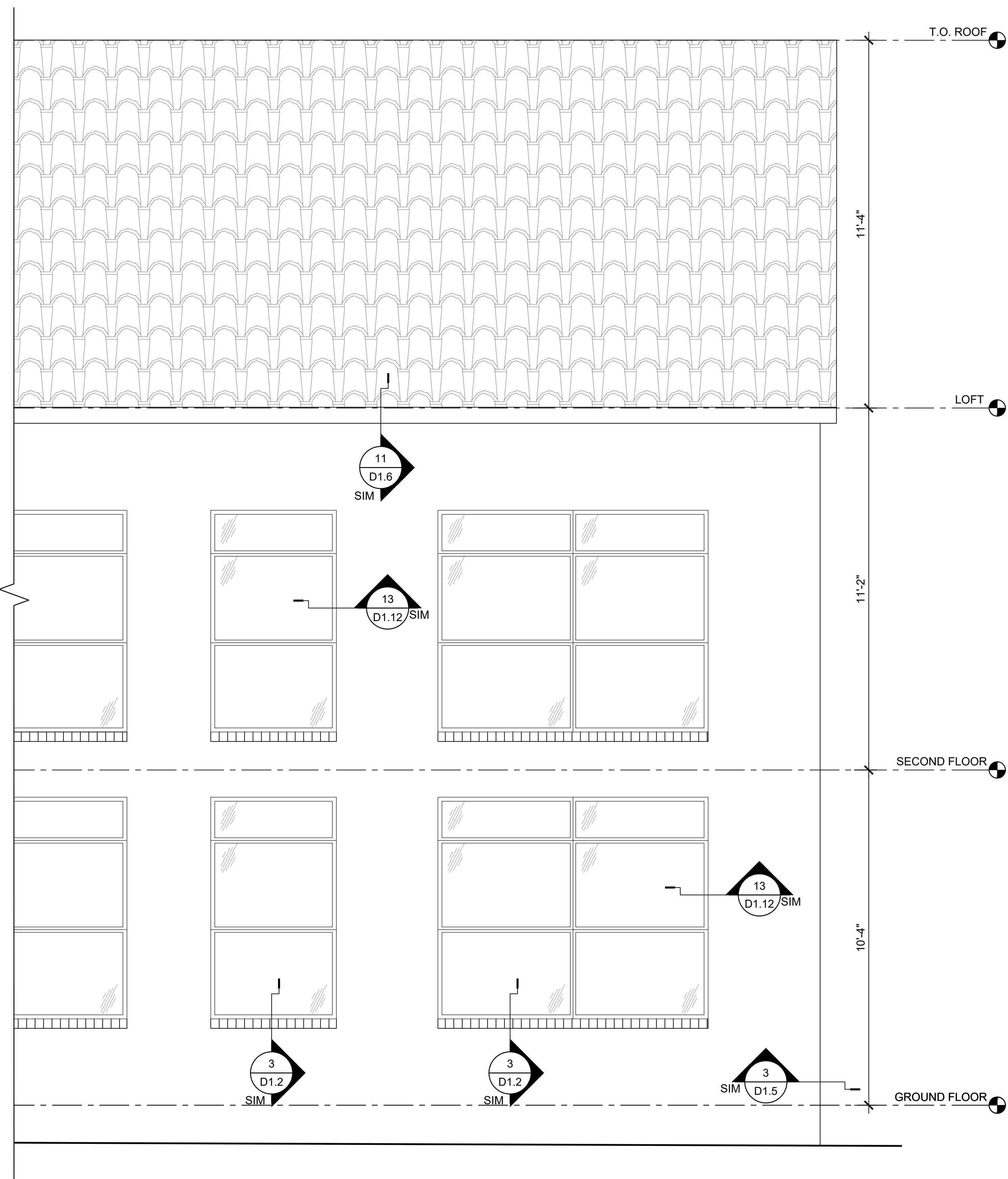
1 BUILDING 5 ELEVATION - WEST SCALE: 1/2"=1'-0"
