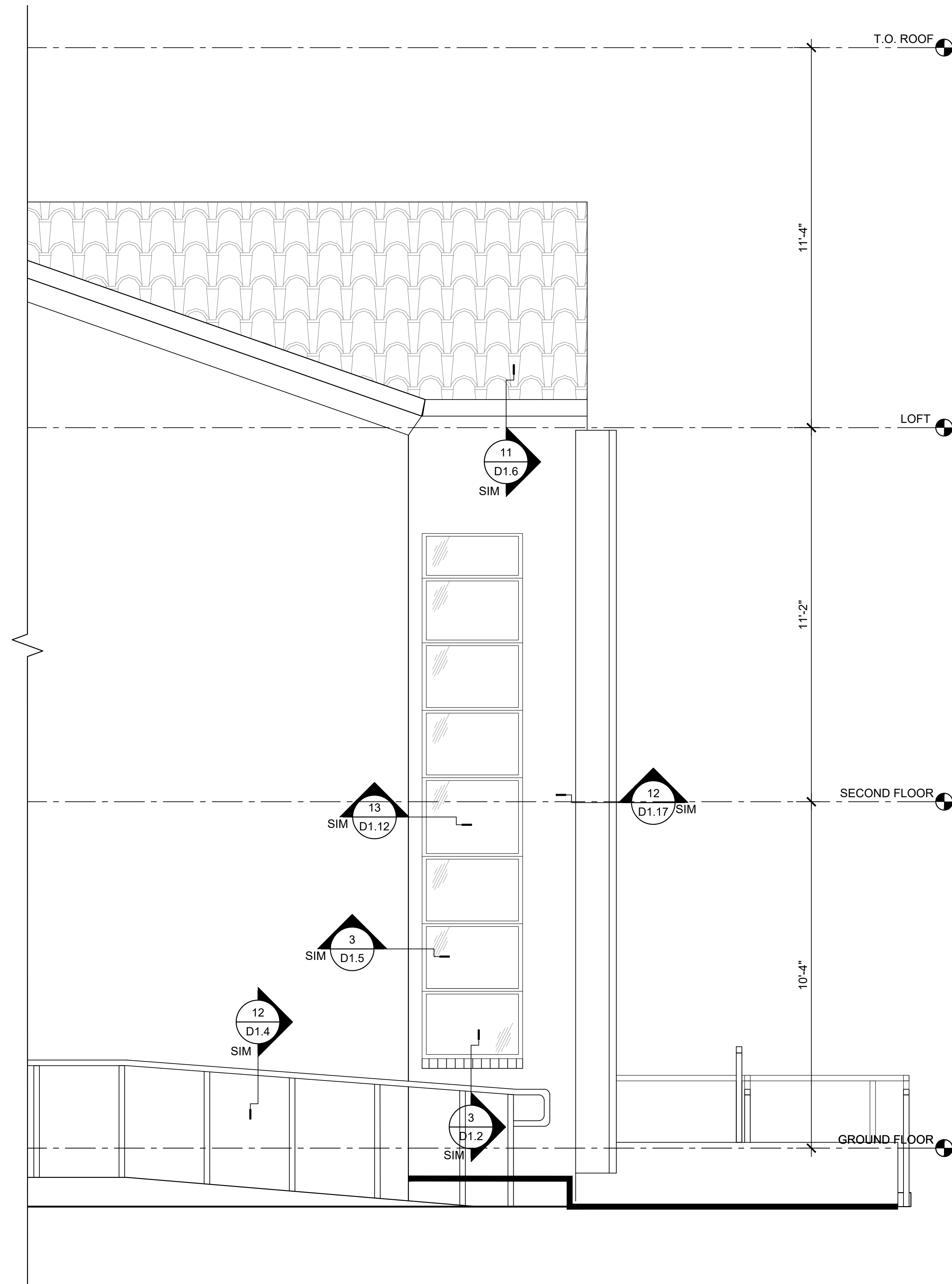
2 BUILDING 5 ELEVATION - NORTH SCALE: 1/2"=1'-0"
