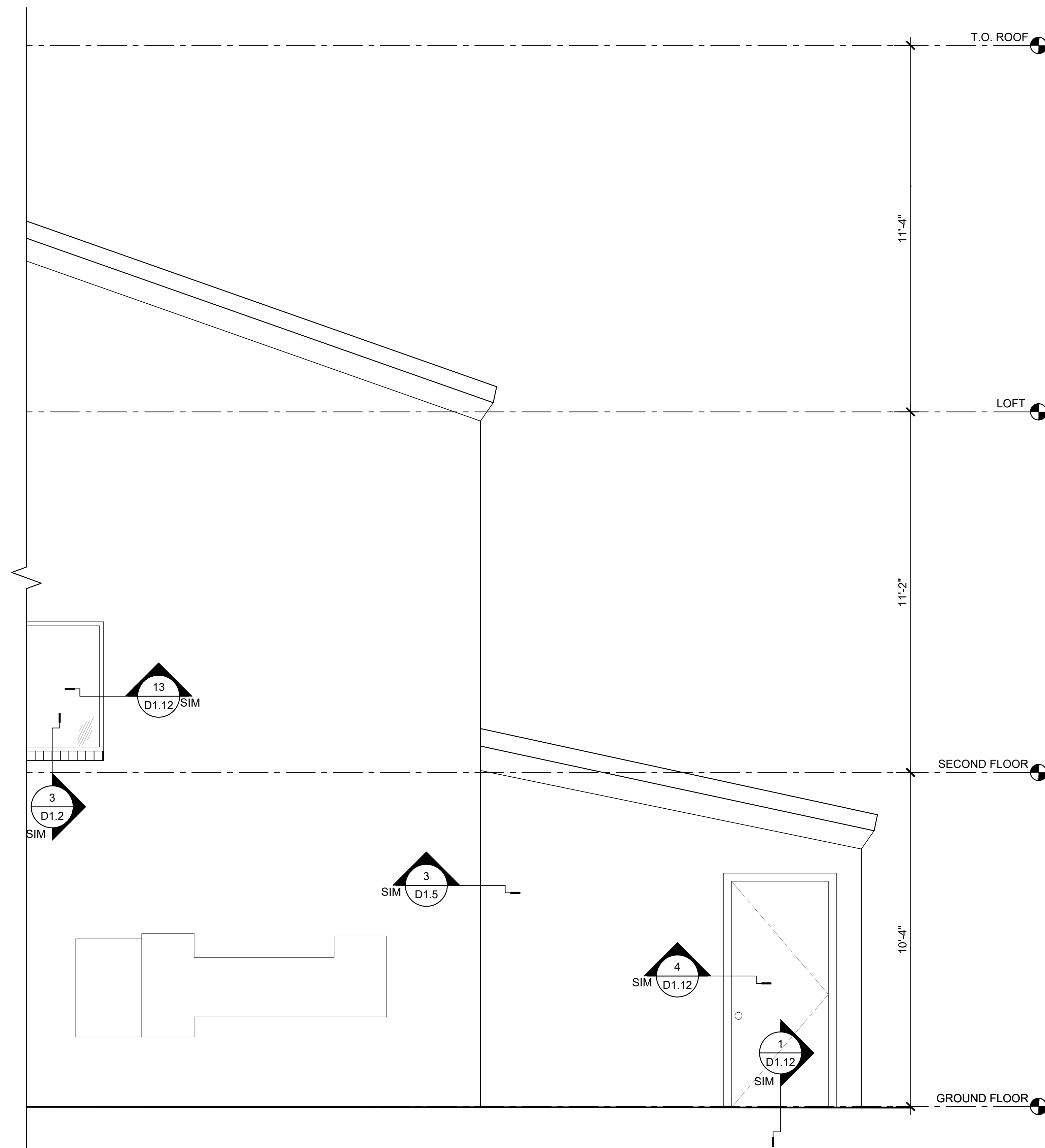
2 BUILDING 5 ELEVATION - SOUTH SCALE: 1/2"=1'-0"
