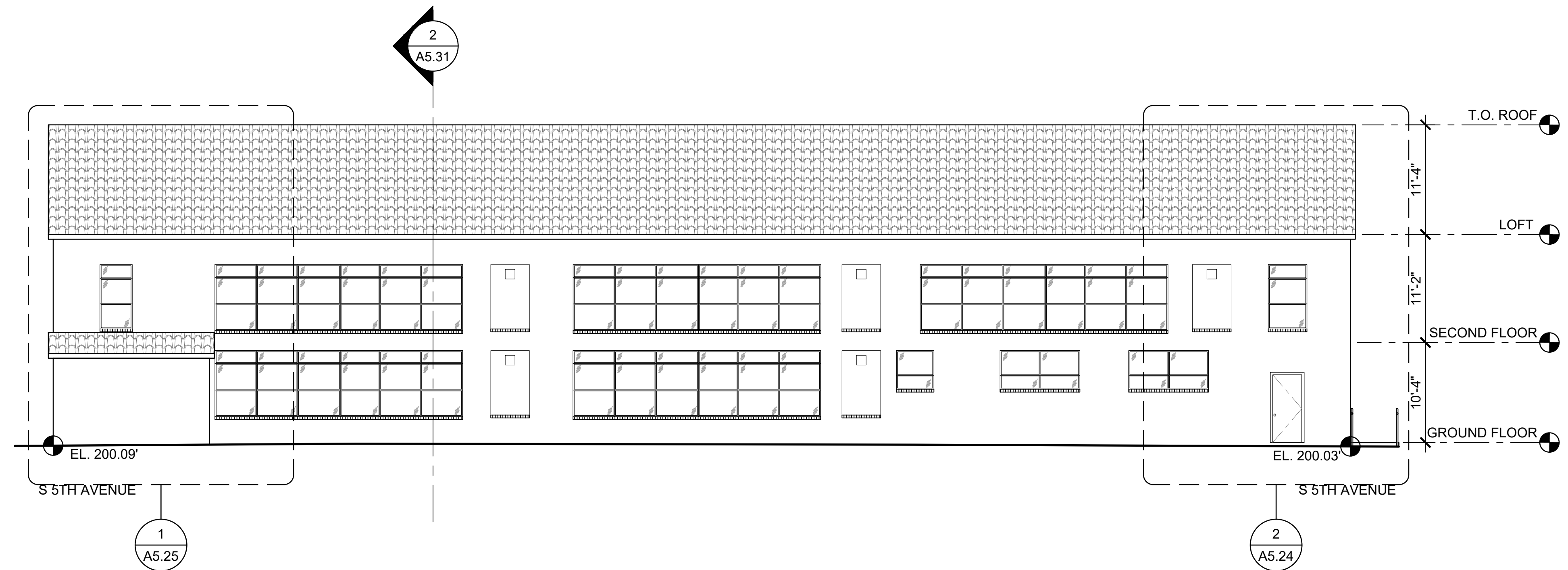
3 BUILDING 5 ELEVATION - EAST SCALE: 1/8"=1'-0"
